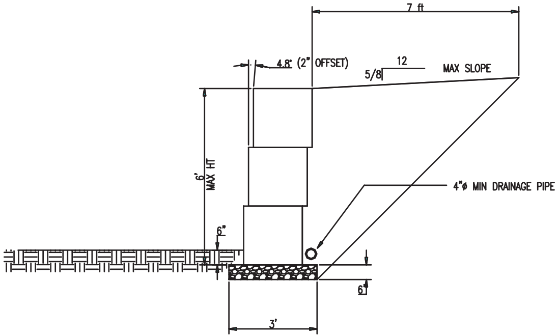
NO SOIL REINFORCEMENT USED
