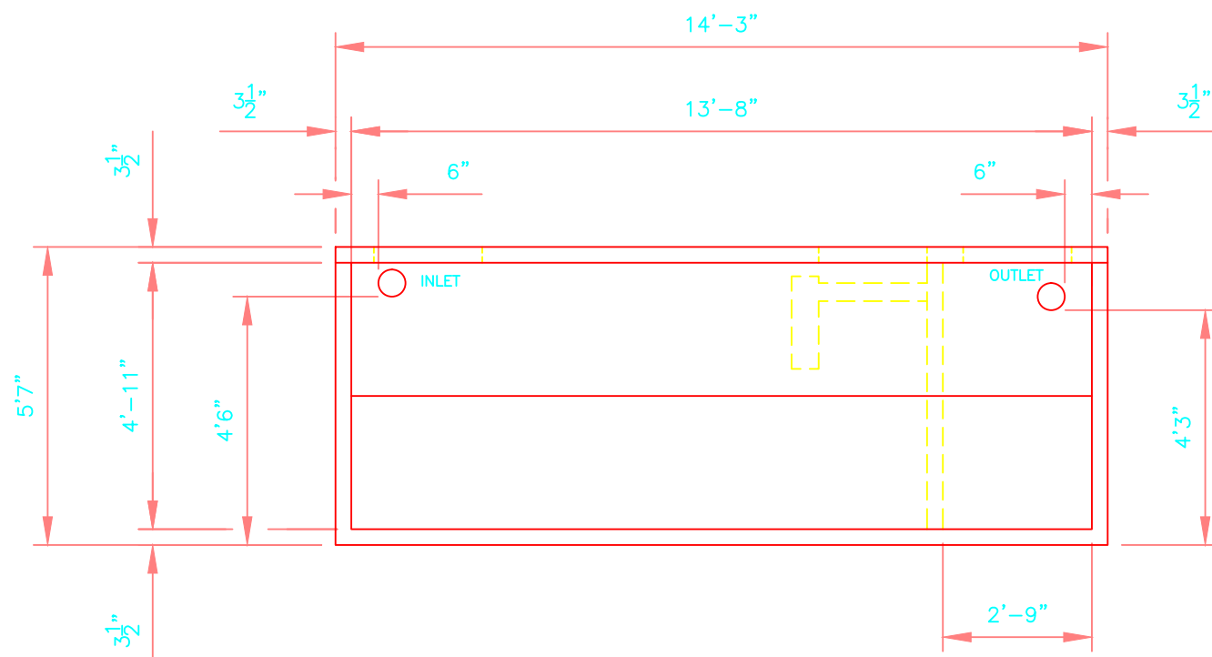
ELEVATION VIEW
