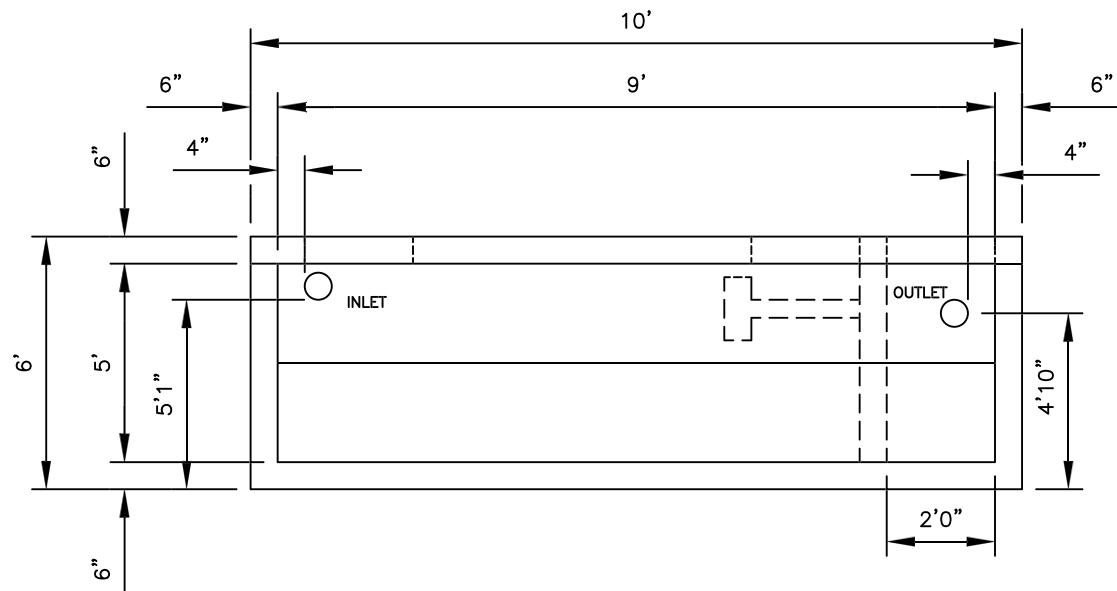
ELEVATION VIEW
