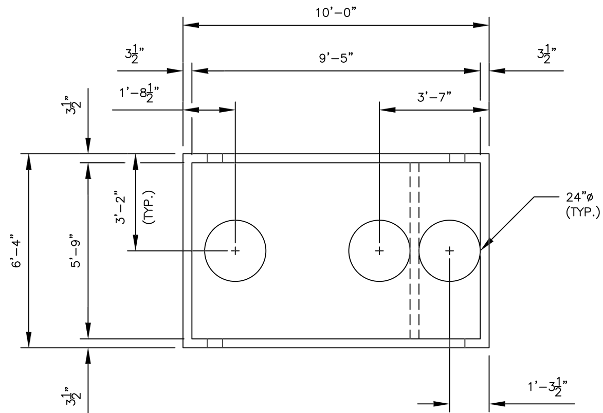
PLAN VIEW
